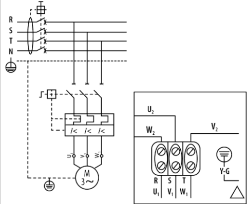
230 Vac - 50 Hz
